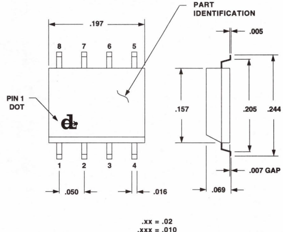
8 PIN PLASTIC
