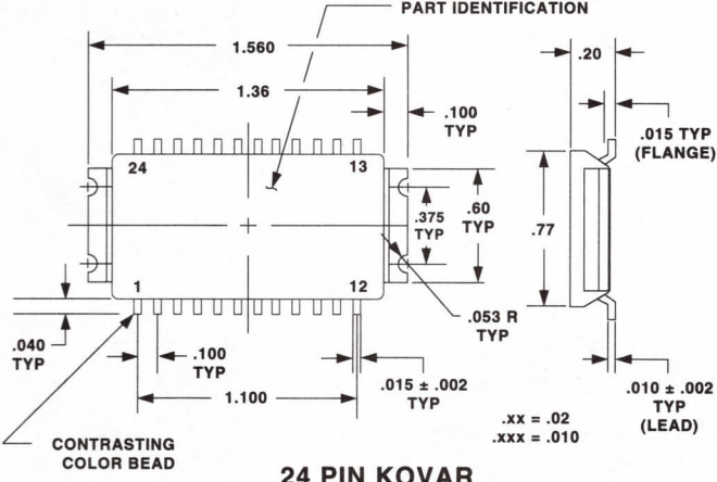
24 PIN KOVAR
