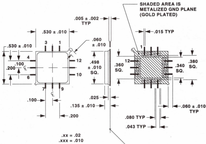
12 PIN CERAMIC/KOVAR
