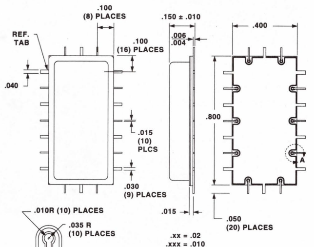
20 PIN CERAMIC/KOVAR (10 GND PINS)
