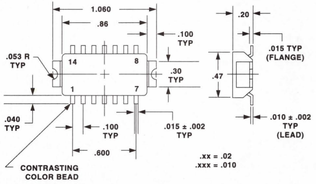
14 PIN KOVAR
