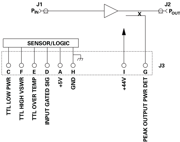
DRIVER / HPA PWR CONN PINOUTS P/N AMP 97 3102A-20-16P
